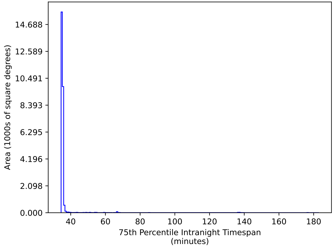
weather_cloudso0v3.5_10yrs All sky iz bands: 75th Percentile Intranight Timespan
