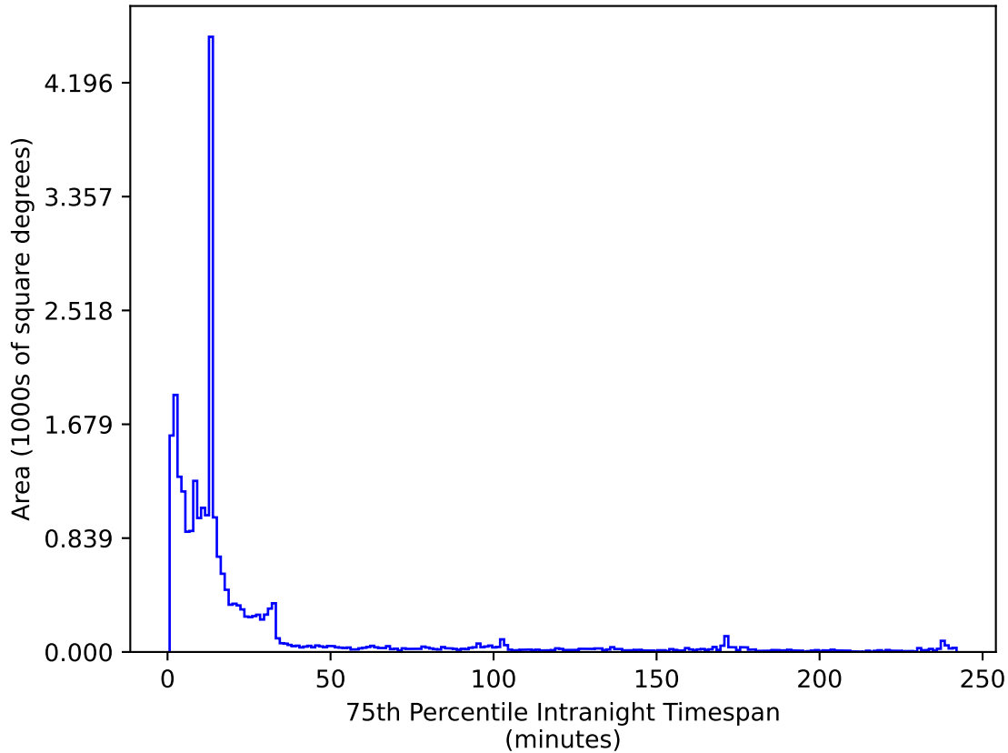
weather_cloudso0v3.5_10yrs All sky i band: 75th Percentile Intranight Timespan
