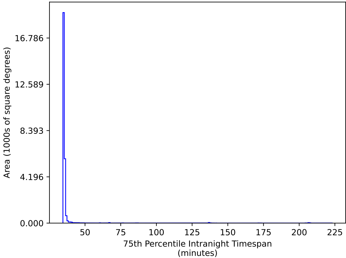
weather_cloudso0v3.5_10yrs All sky gr bands: 75th Percentile Intranight Timespan
