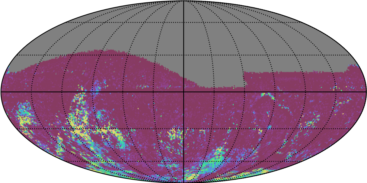
weather_cloudso0v3.5_10yrs All sky g band: 75th Percentile Intranight Timespan
