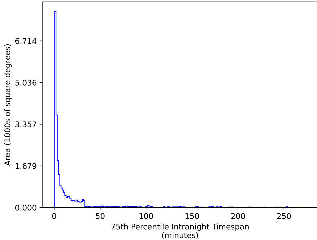
weather_cloudso0v3.5_10yrs All sky g band: 75th Percentile Intranight Timespan
