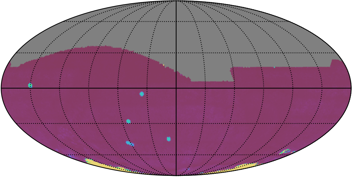
weather_cloudso0v3.5_10yrs All sky all bands: 75th Percentile Intranight Timespan
