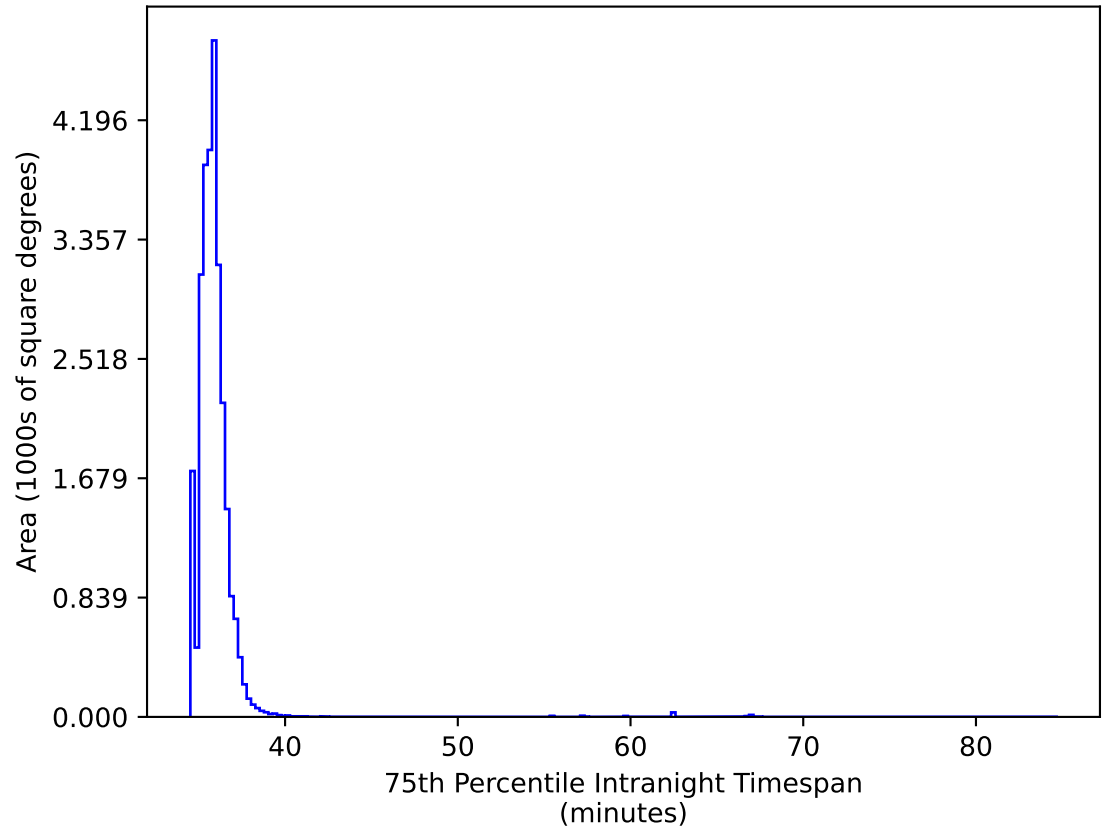
weather_cloudso0v3.5_10yrs All sky all bands: 75th Percentile Intranight Timespan
