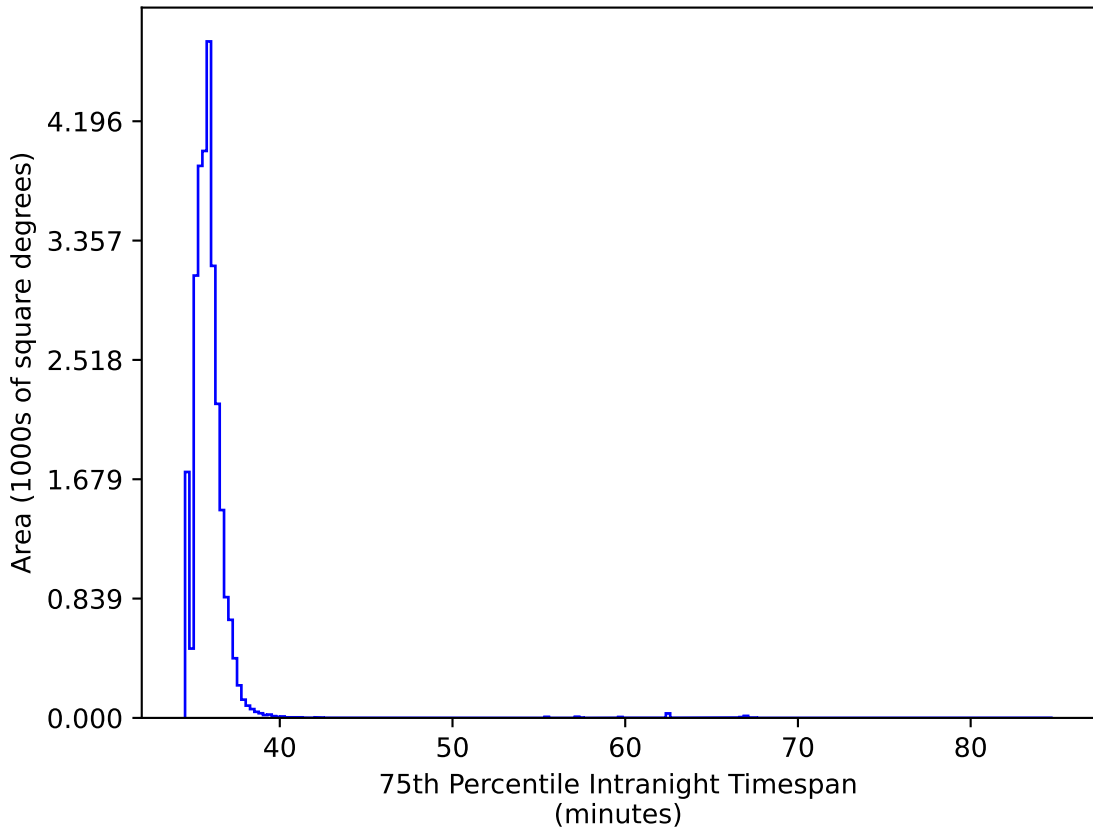
weather_cloudso0v3.5_10yrs All sky: 75th Percentile Intranight Timespan
