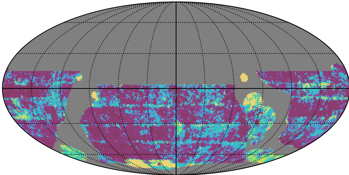
weather_cloudso0v3.5_10yrs WFD z band: 20thPercentile Inter-Night Gap
