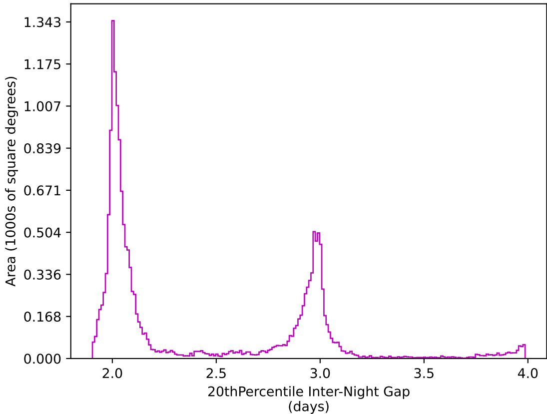
weather_cloudso0v3.5_10yrs WFD z band: 20thPercentile Inter-Night Gap
