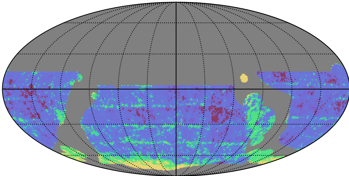
weather_cloudso0v3.5_10yrs WFD r band: 20thPercentile Inter-Night Gap
