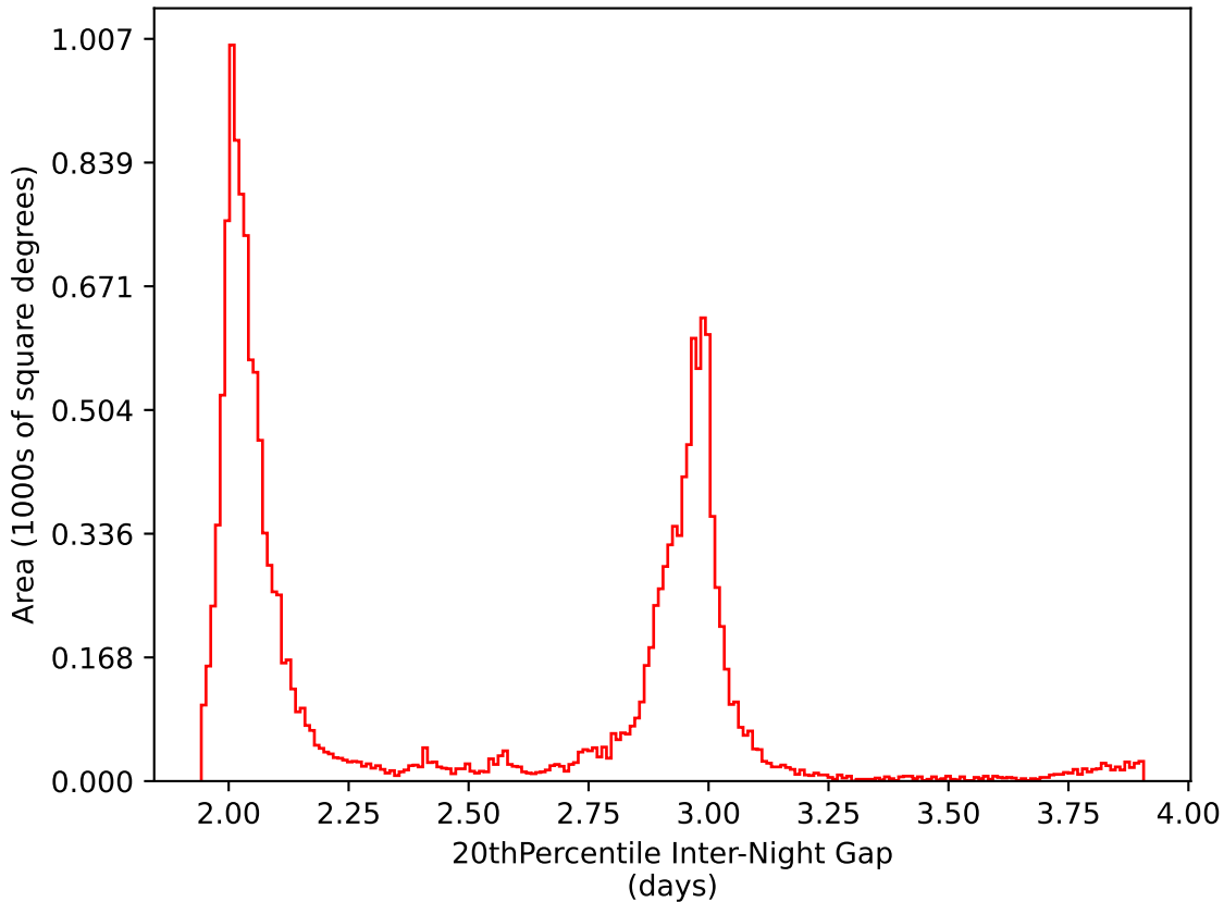
weather_cloudso0v3.5_10yrs WFD i band: 20thPercentile Inter-Night Gap
