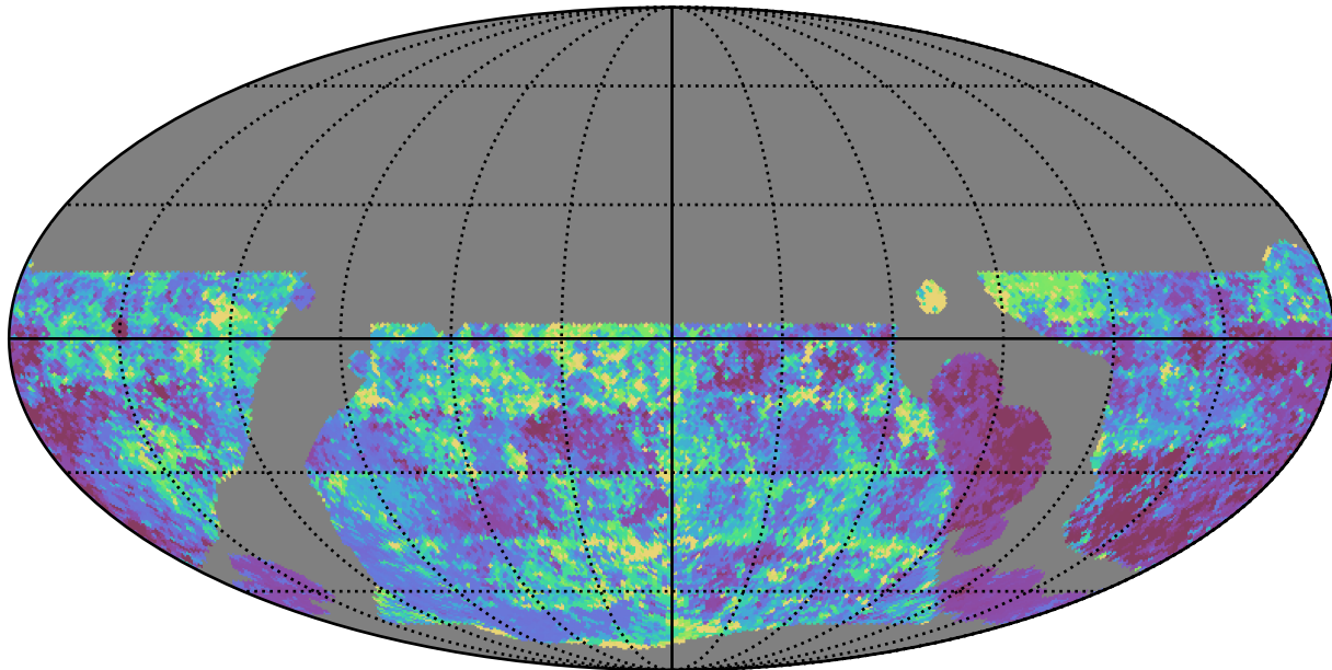
weather_cloudso0v3.5_10yrs WFD g band: 20thPercentile Inter-Night Gap
