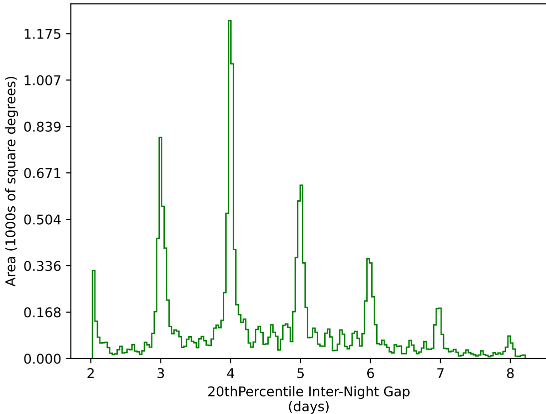
weather_cloudso0v3.5_10yrs WFD g band: 20thPercentile Inter-Night Gap
