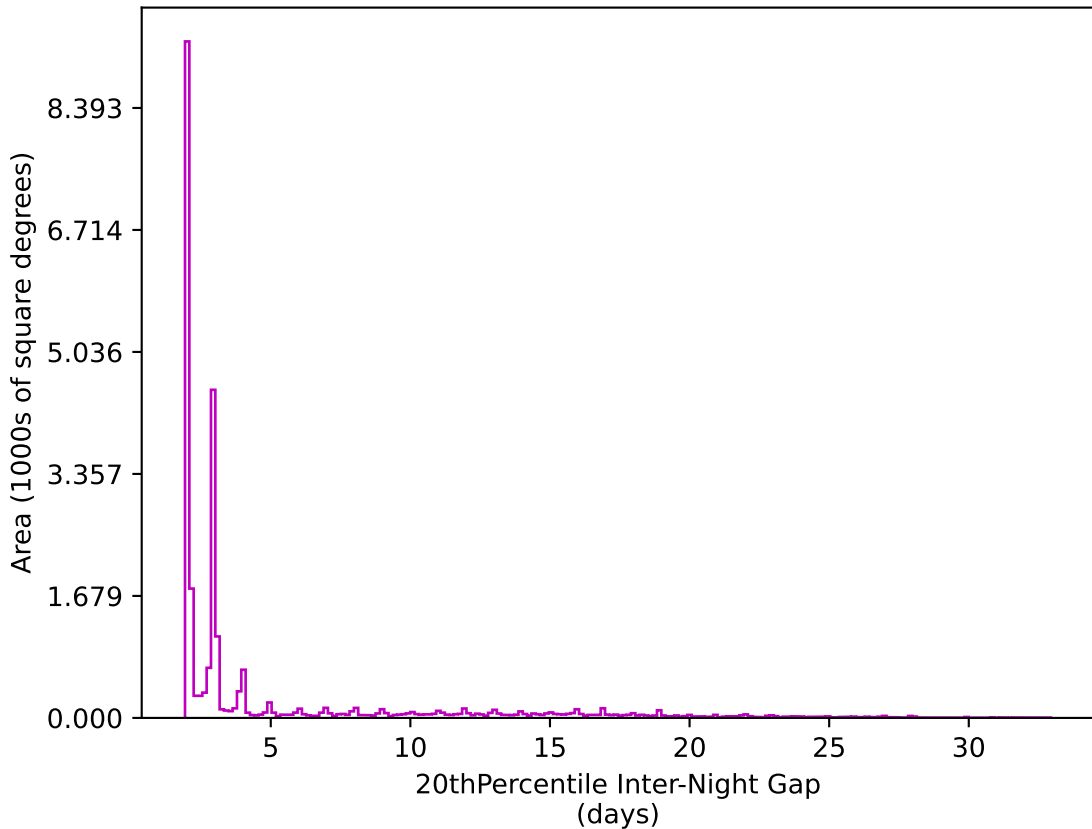
weather_cloudso0v3.5_10yrs All sky z band: 20thPercentile Inter-Night Gap
