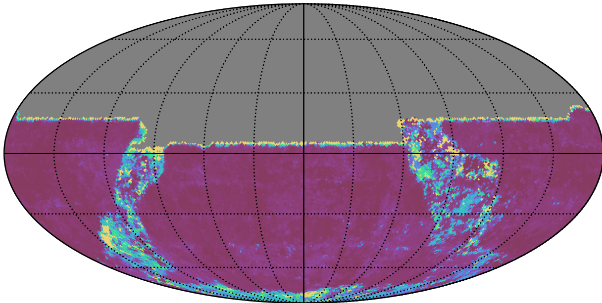
weather_cloudso0v3.5_10yrs All sky u band: 20thPercentile Inter-Night Gap
