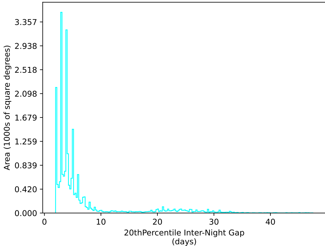
weather_cloudso0v3.5_10yrs All sky u band: 20thPercentile Inter-Night Gap
