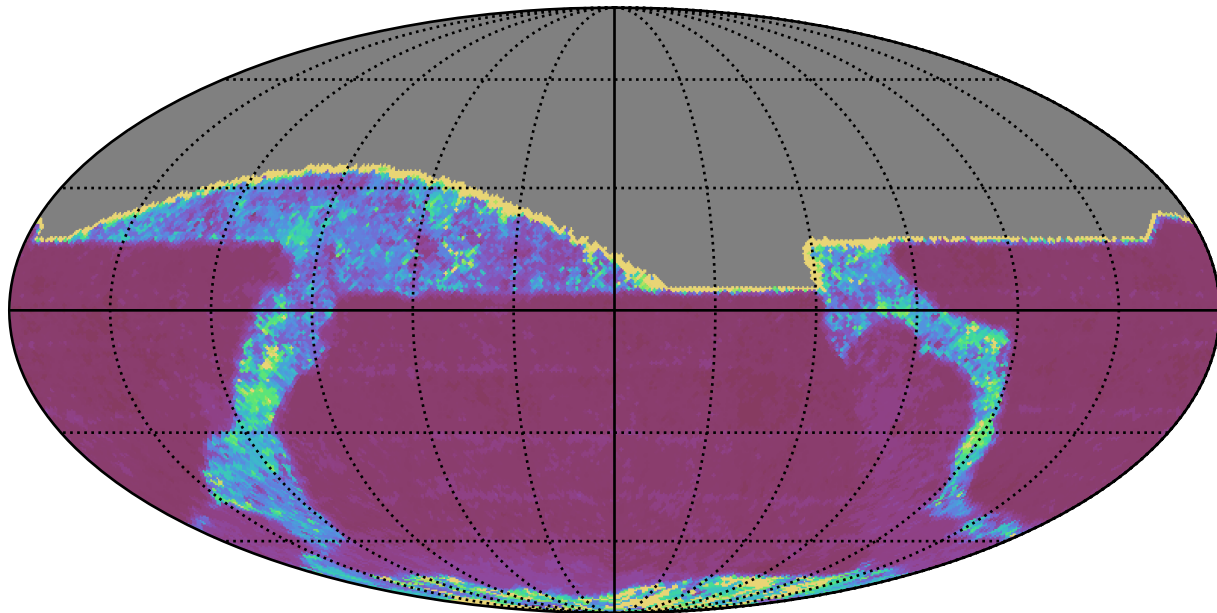
weather_cloudso0v3.5_10yrs All sky r band: 20thPercentile Inter-Night Gap
