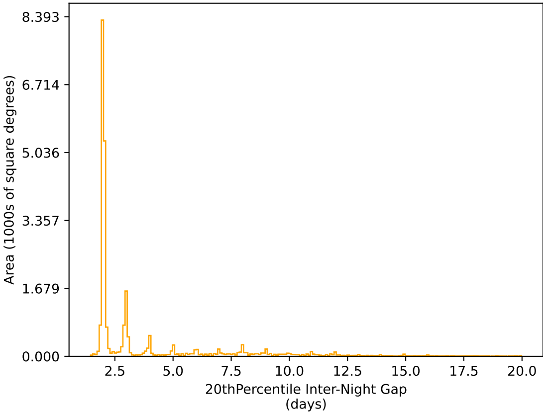
weather_cloudso0v3.5_10yrs All sky r band: 20thPercentile Inter-Night Gap
