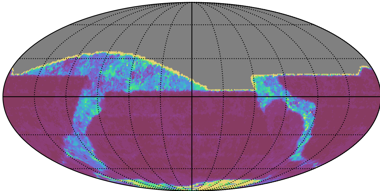
weather_cloudso0v3.5_10yrs All sky i band: 20thPercentile Inter-Night Gap
