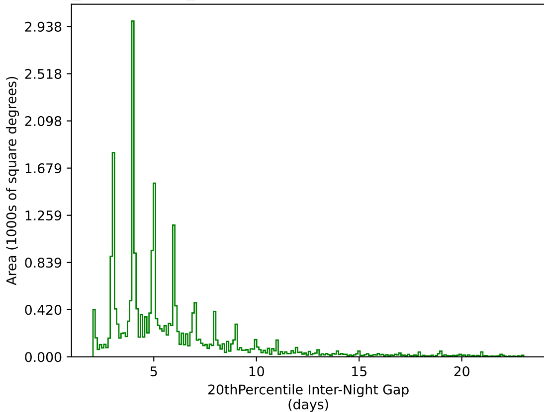
weather_cloudso0v3.5_10yrs All sky g band: 20thPercentile Inter-Night Gap
