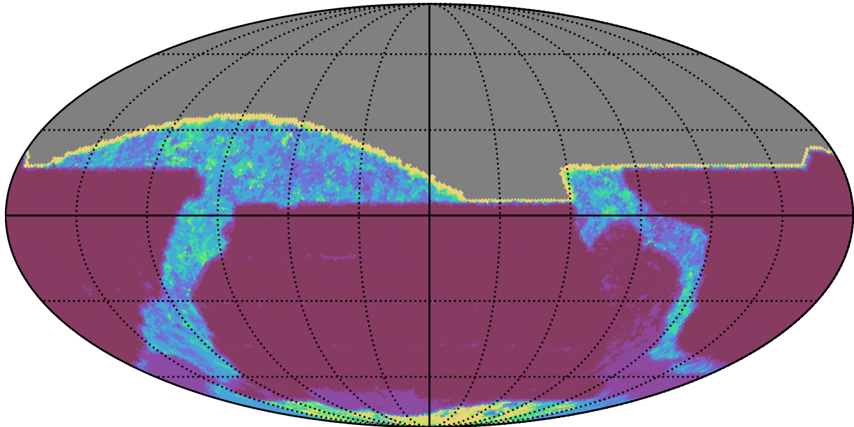
weather_cloudso0v3.5_10yrs All sky all bands: 20thPercentile Inter-Night Gap
