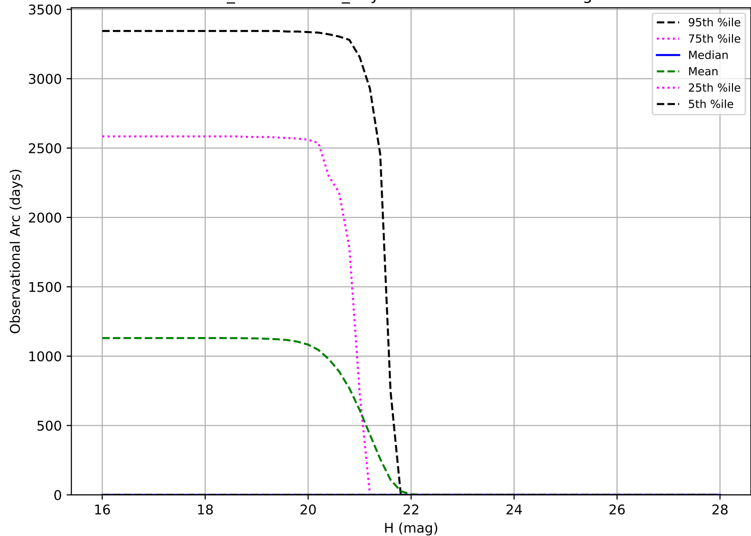
weather_cloudso0v3.4_10yrs: Observational Arc Length Vatira
