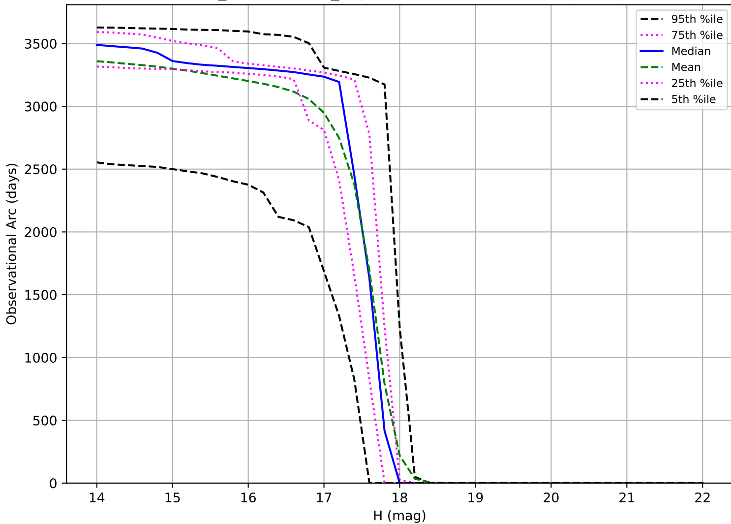
weather_cloudso0v3.4_10yrs: Observational Arc Length Trojan
