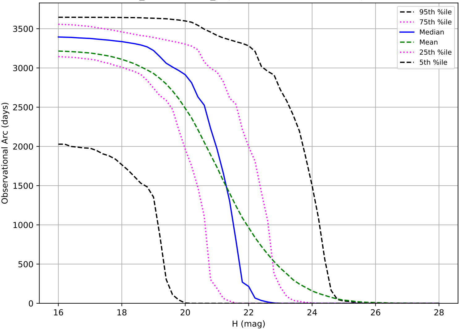
weather_cloudso0v3.4_10yrs: Observational Arc Length PHA
