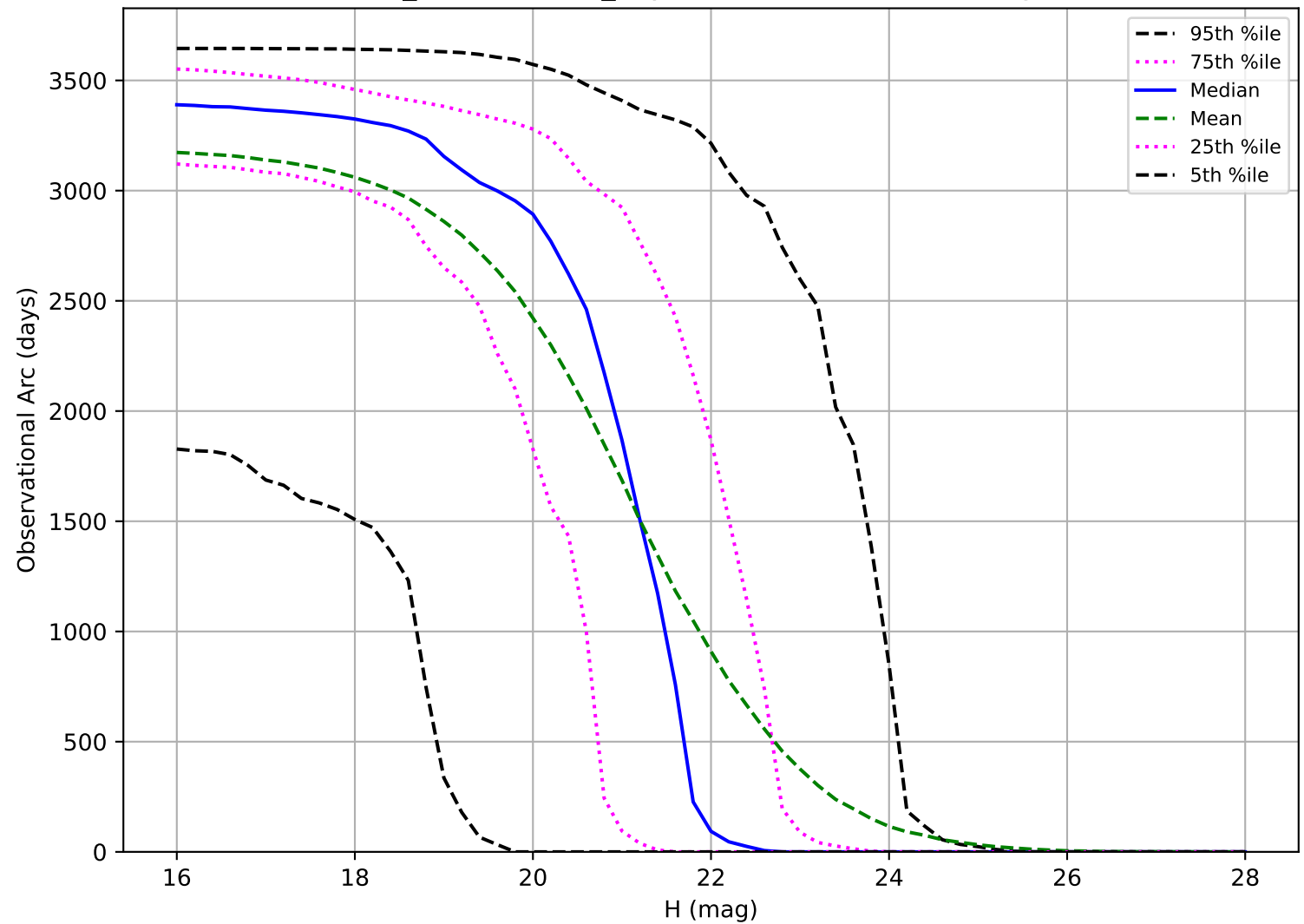
weather_cloudso0v3.4_10yrs: Observational Arc Length NEO
