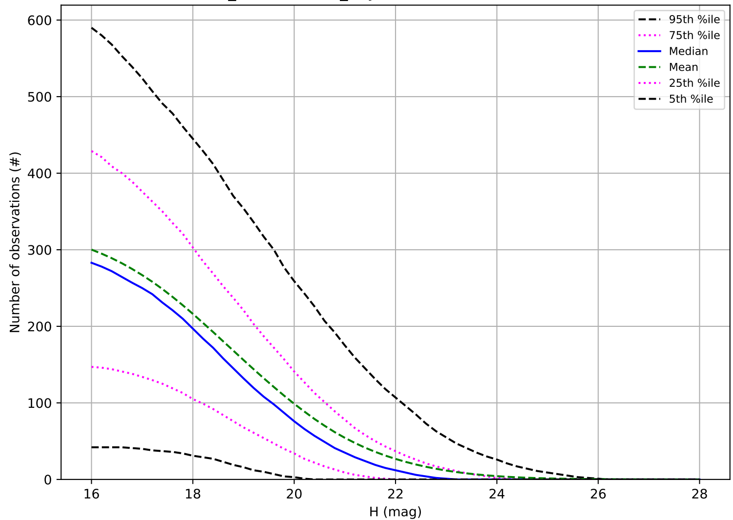
weather_cloudso0v3.4_10yrs: Number of observations PHA
