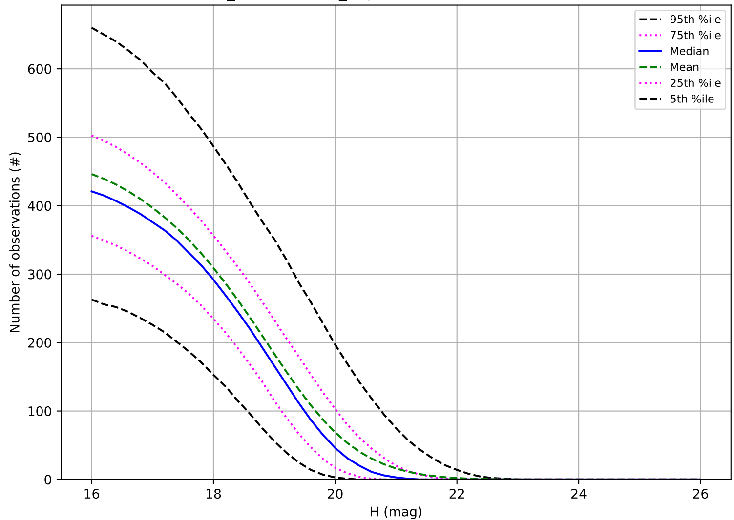
weather_cloudso0v3.4_10yrs: Number of observations MBA
