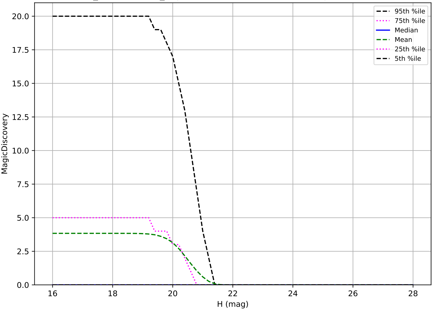
weather_cloudso0v3.4_10yrs: Vatira 6 detections in 60 nights detection loss
