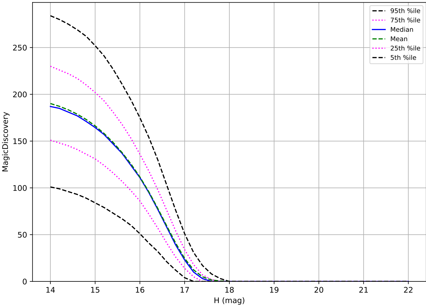
weather_cloudso0v3.4_10yrs: Trojan 6 detections in 60 nights detection loss
