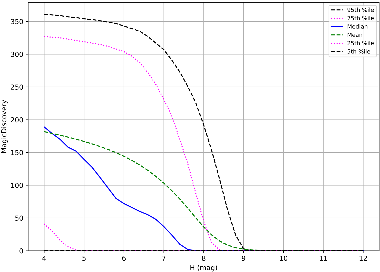
weather_cloudso0v3.4_10yrs: TNO 6 detections in 60 nights detection loss
