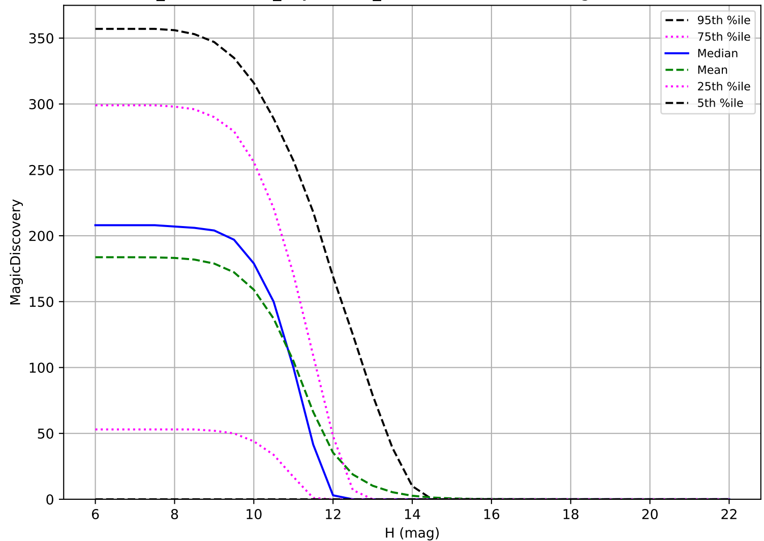
weather_cloudso0v3.4_10yrs: OCC_r20 6 detections in 60 nights detection loss
