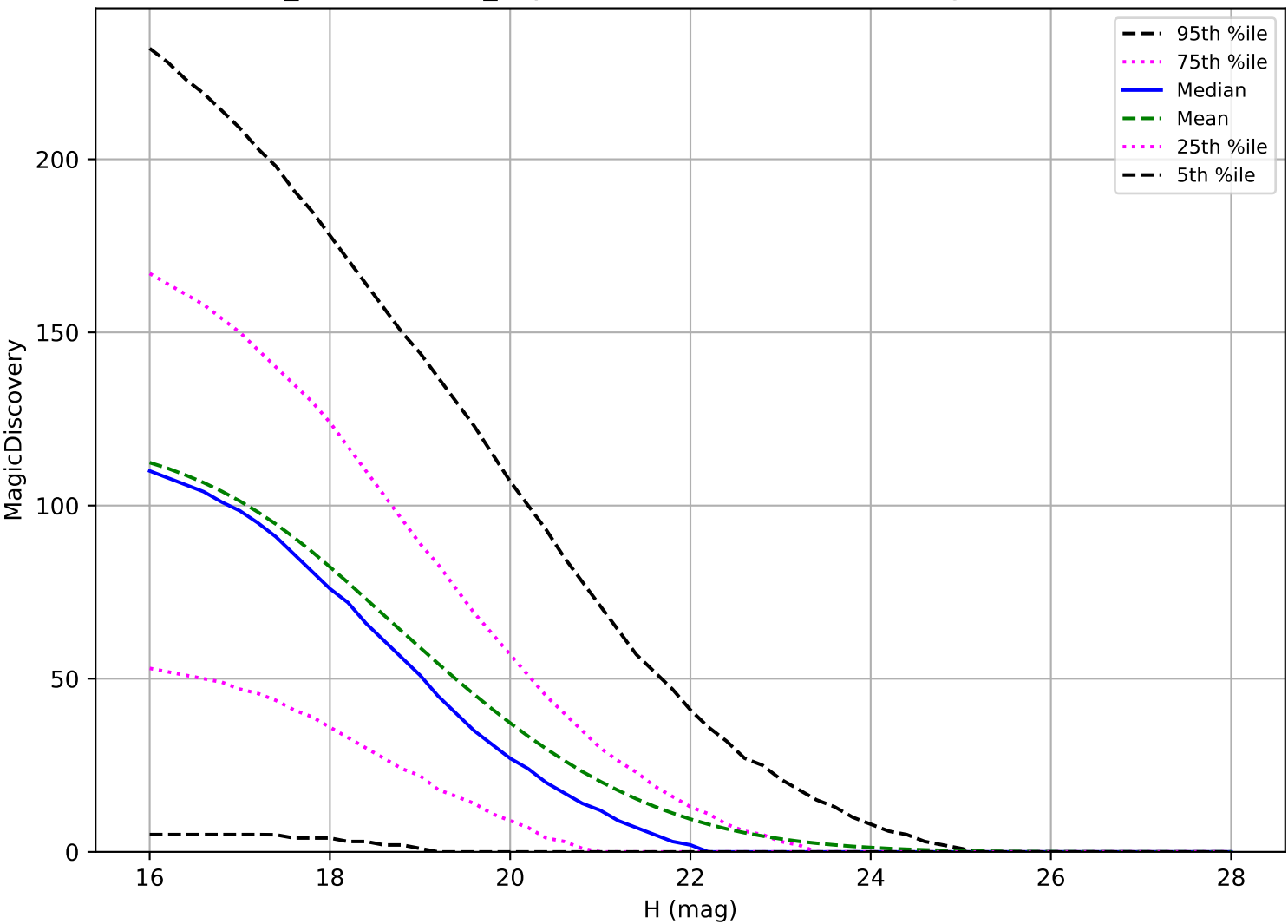
weather_cloudso0v3.4_10yrs: NEO 6 detections in 60 nights detection loss
