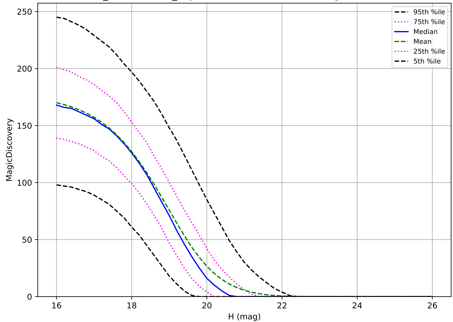
weather_cloudso0v3.4_10yrs: MBA 6 detections in 60 nights detection loss
