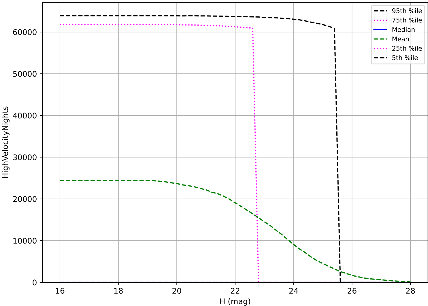
weather_cloudso0v3.4_10yrs: PHA High velocity pair detection loss
