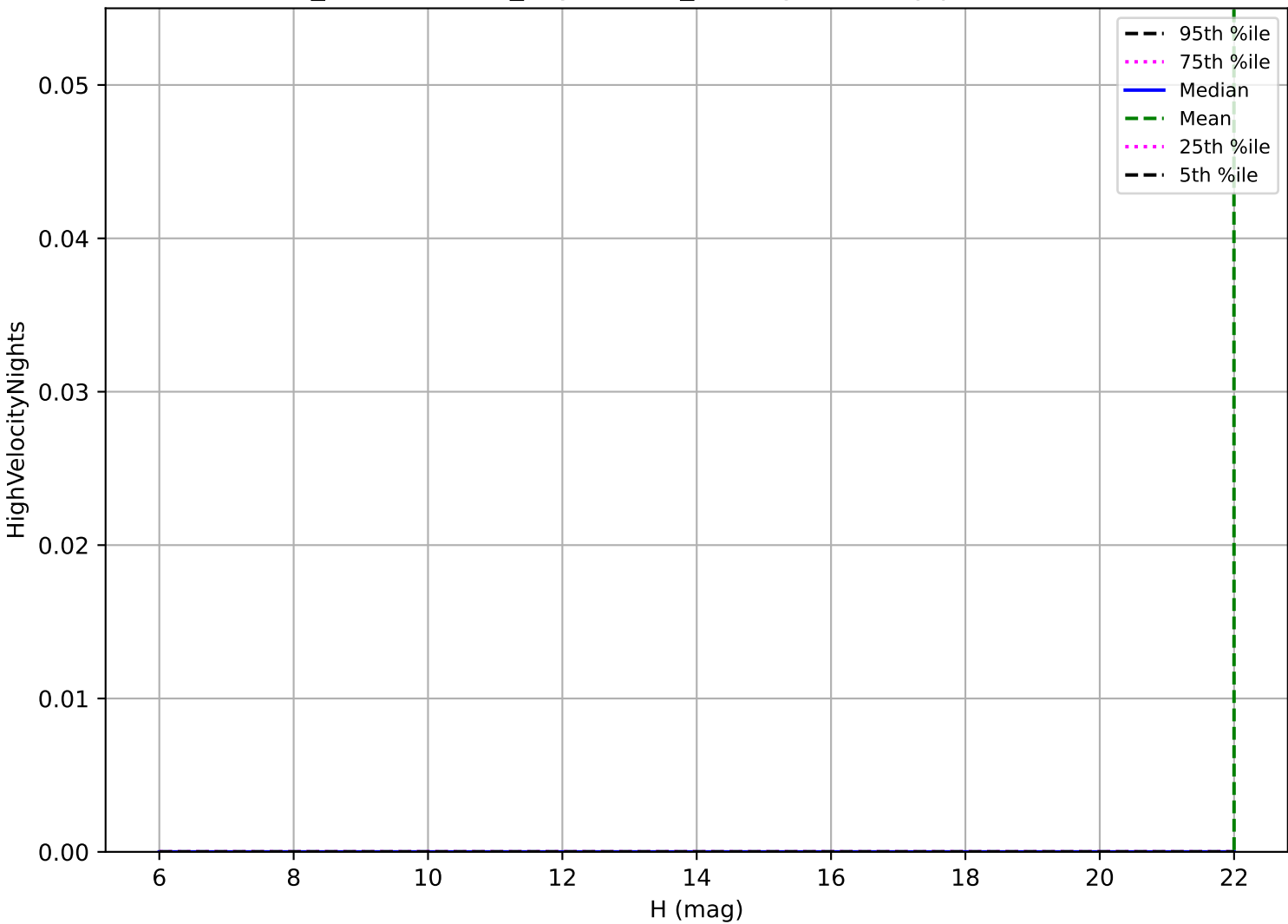
weather_cloudso0v3.4_10yrs: OCC_r20 High velocity pair detection loss
