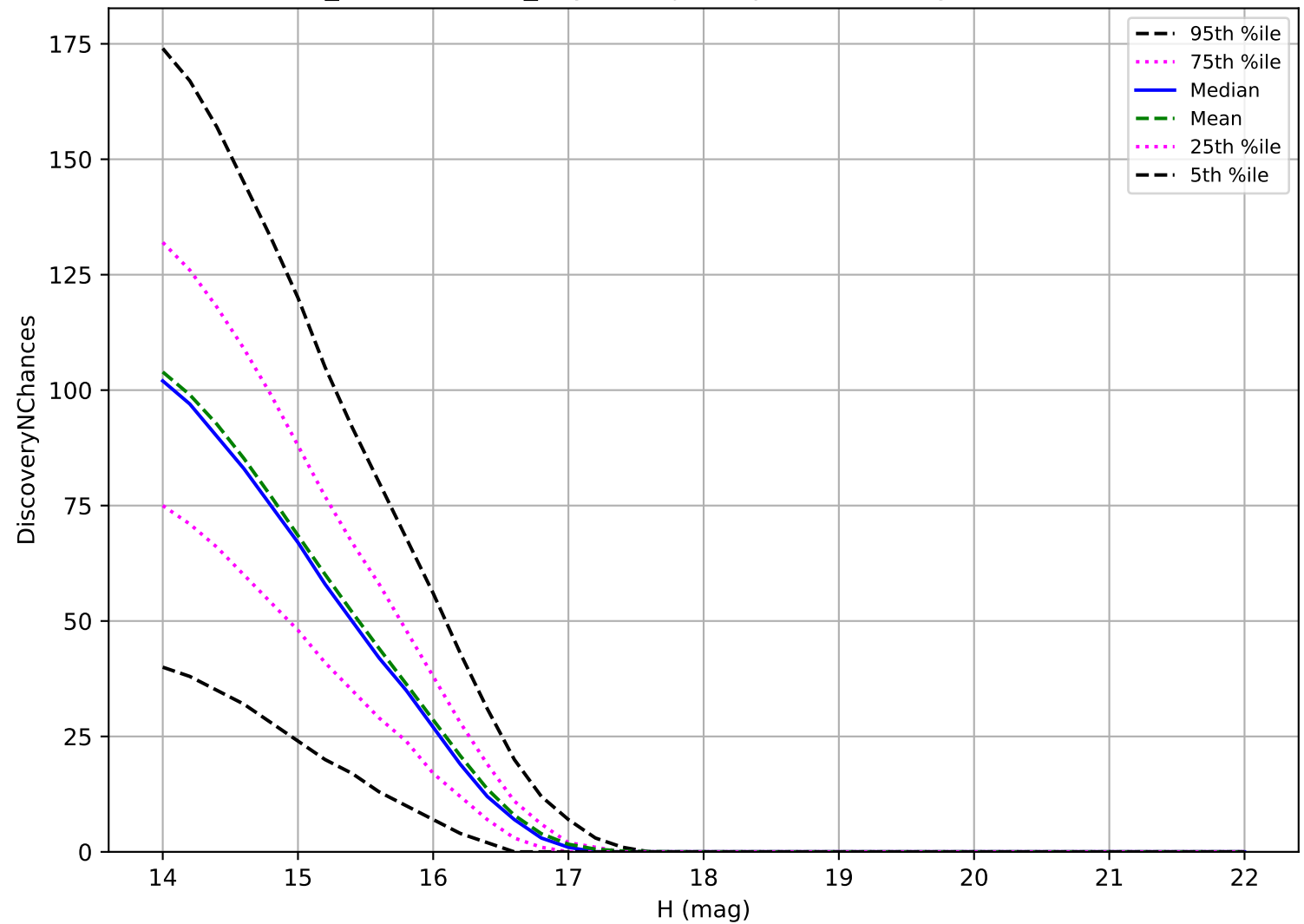
weather_cloudso0v3.4_10yrs: Trojan 3 pairs in 15 nights detection loss
