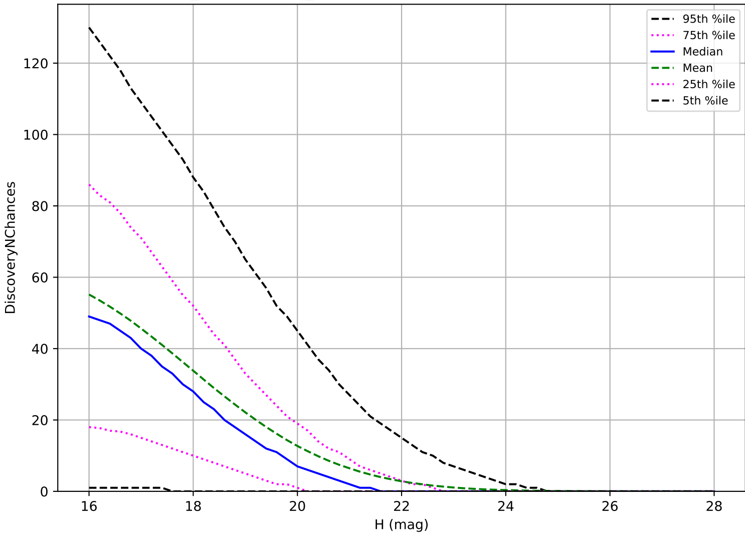
weather_cloudso0v3.4_10yrs: PHA 3 pairs in 15 nights detection loss
