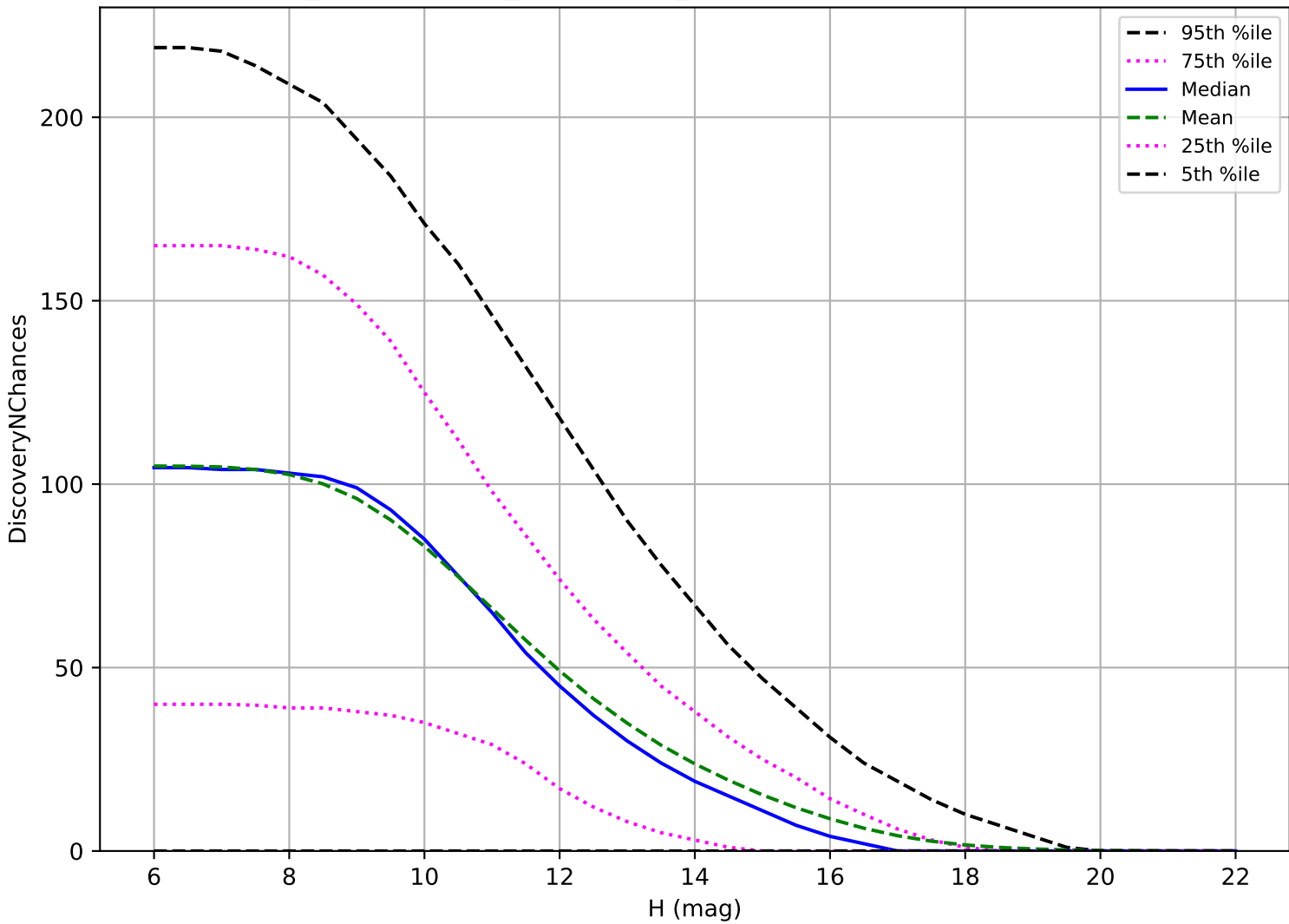
weather_cloudso0v3.4_10yrs: OCC_r5 3 pairs in 15 nights detection loss
