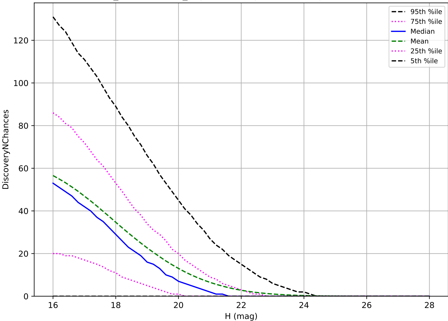
weather_cloudso0v3.4_10yrs: NEO 3 pairs in 15 nights detection loss
