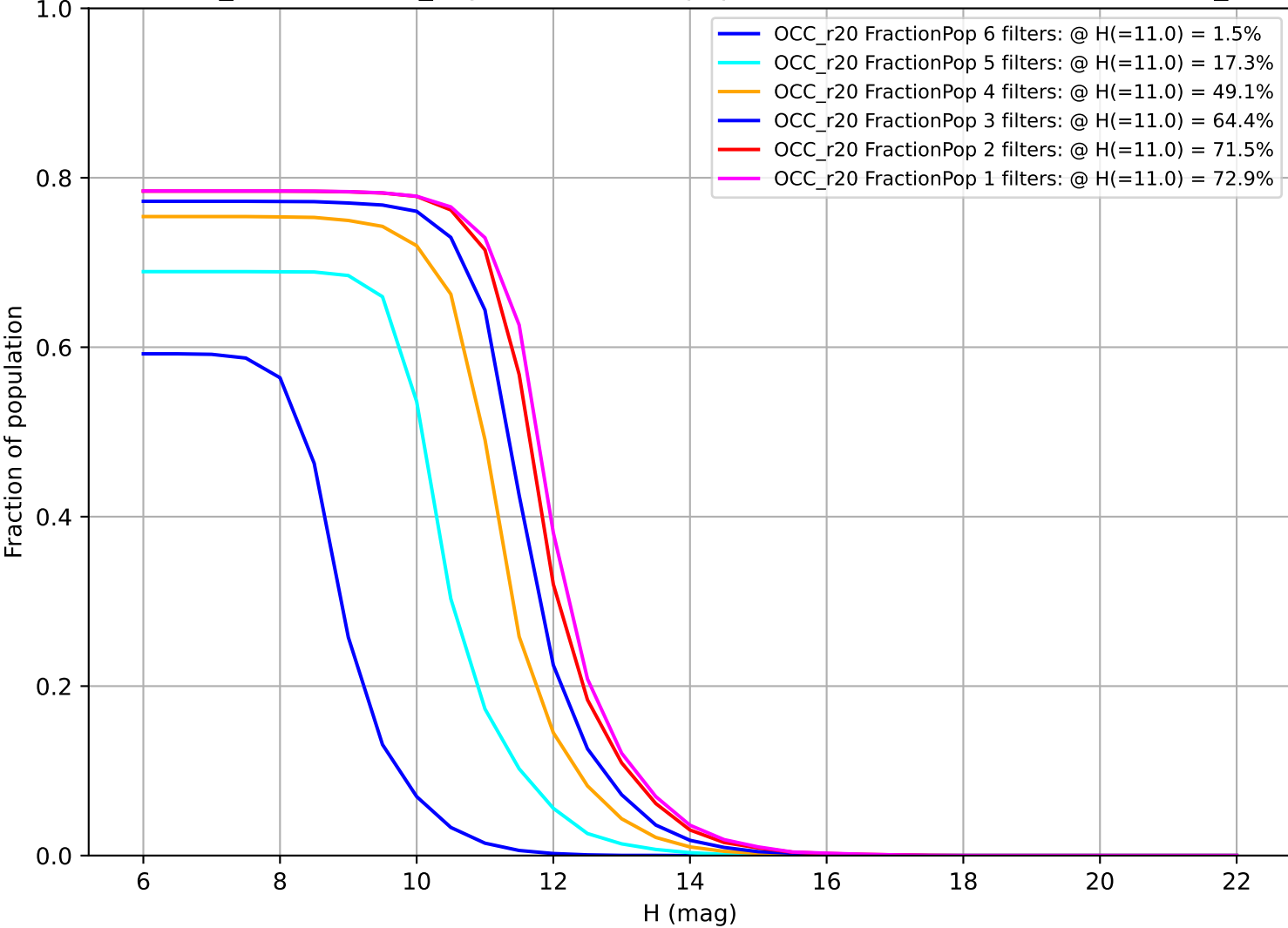
weather_cloudso0v3.4_10yrs: Fraction of population with colors in X filters OCC_r20
