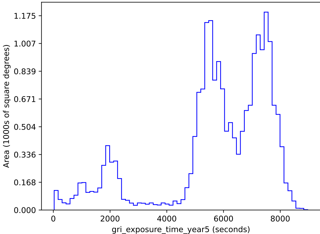
weather_cloudso0v3.4_10yrs gri band non-DD: gri_exposure_time_year5
