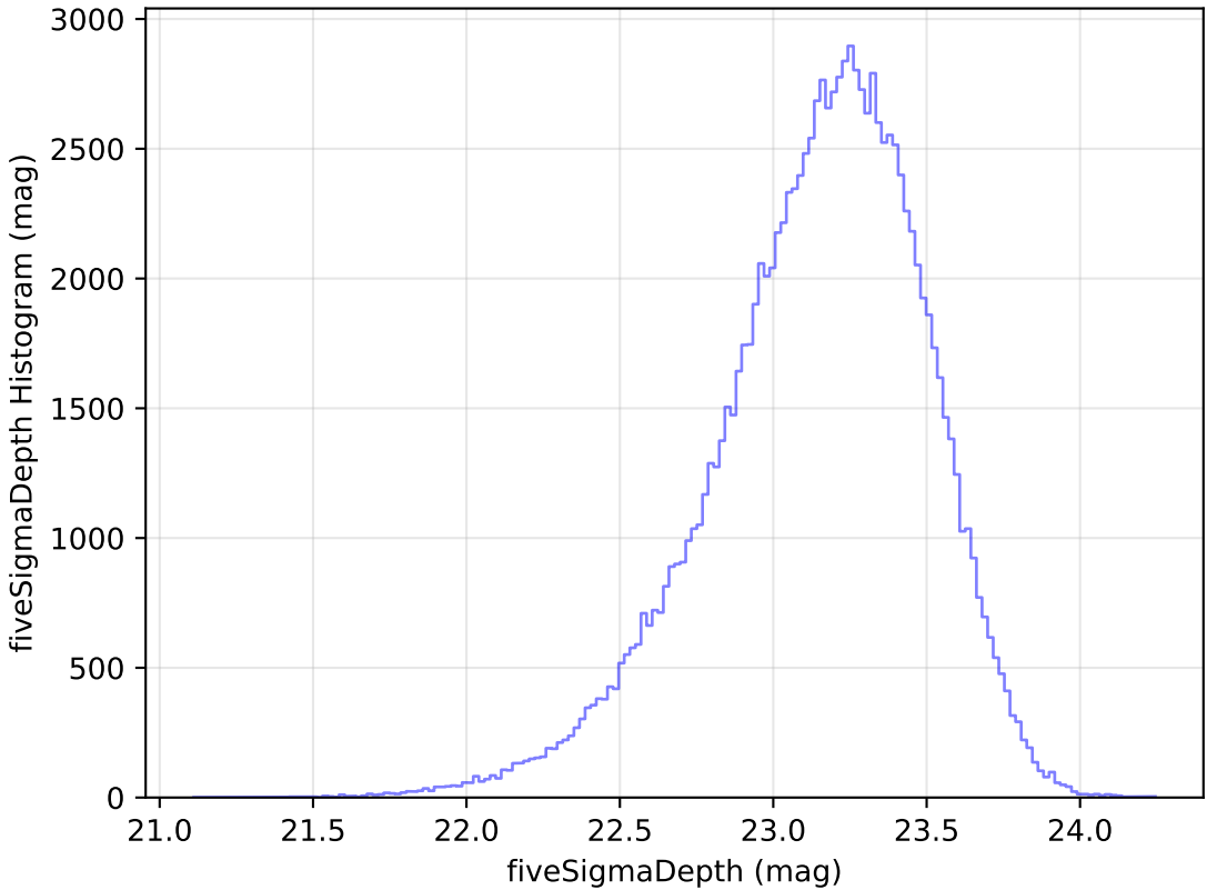
weather_cloudso0v3.4_10yrs u: fiveSigmaDepth Histogram
