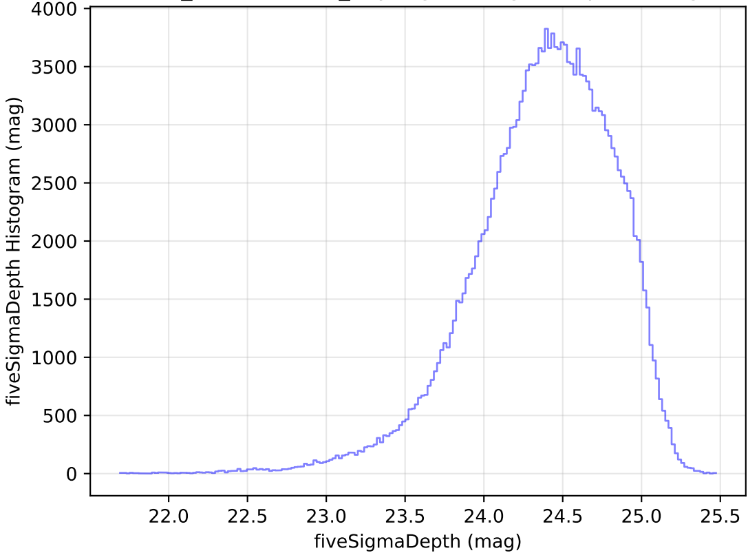
weather_cloudso0v3.4_10yrs g: fiveSigmaDepth Histogram
