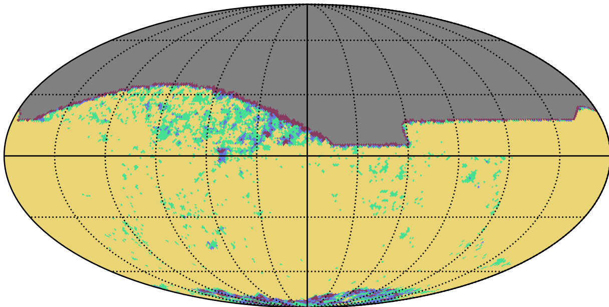
weather_cloudso0v3.4_10yrs z band: YearCoverage night
