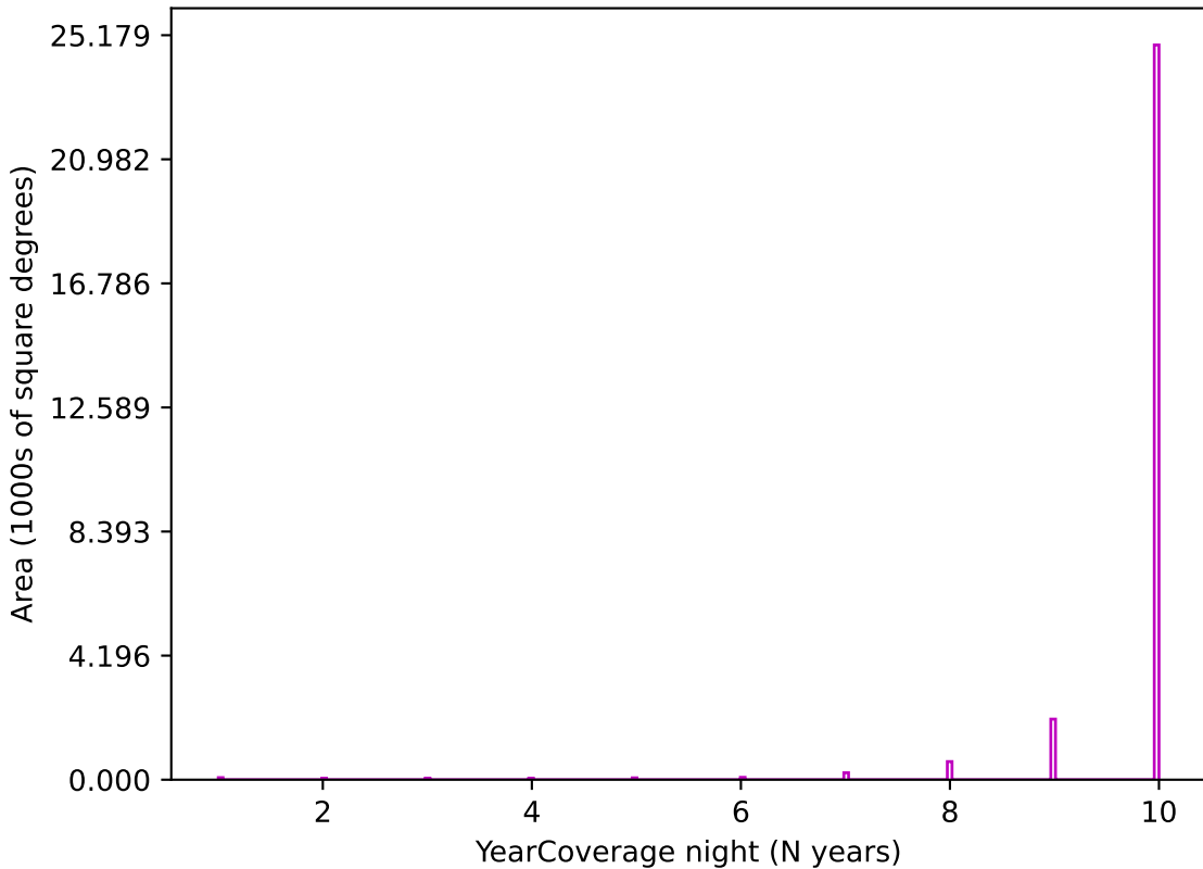
weather_cloudso0v3.4_10yrs z band: YearCoverage night
