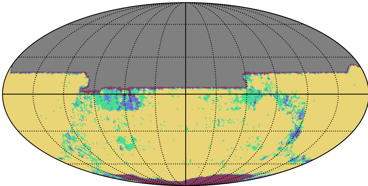
weather_cloudso0v3.4_10yrs y band: YearCoverage night
