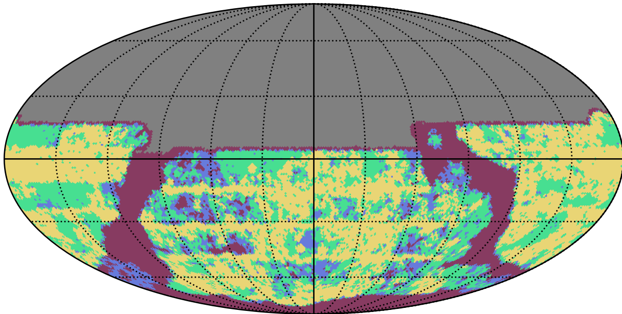
weather_cloudso0v3.4_10yrs u band: YearCoverage night
