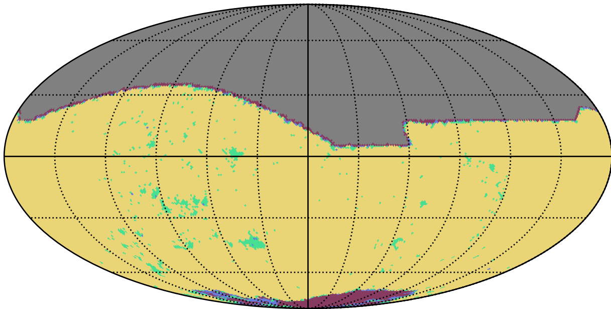
weather_cloudso0v3.4_10yrs r band: YearCoverage night
