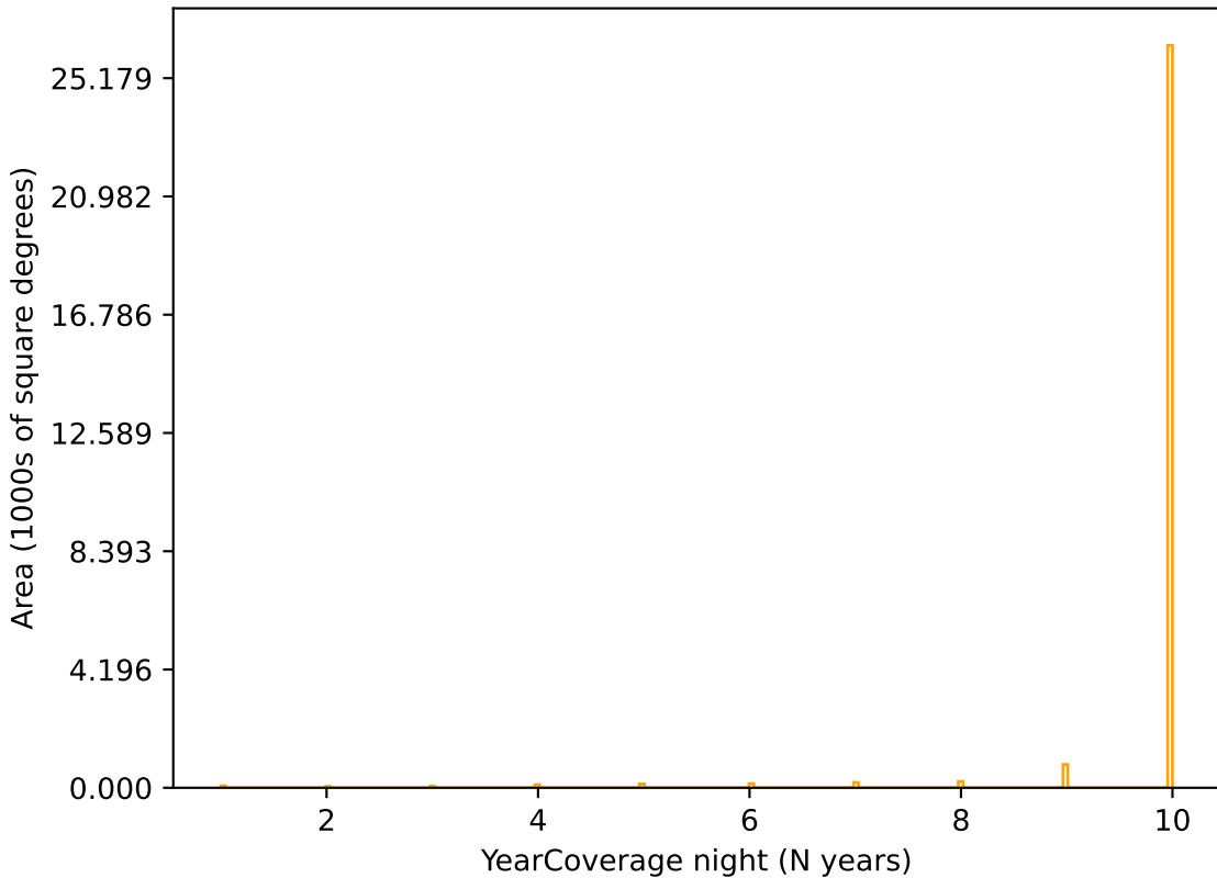
weather_cloudso0v3.4_10yrs r band: YearCoverage night
